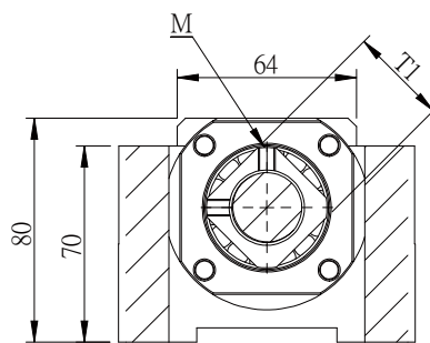
Section U-U
