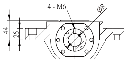
Section U-U
