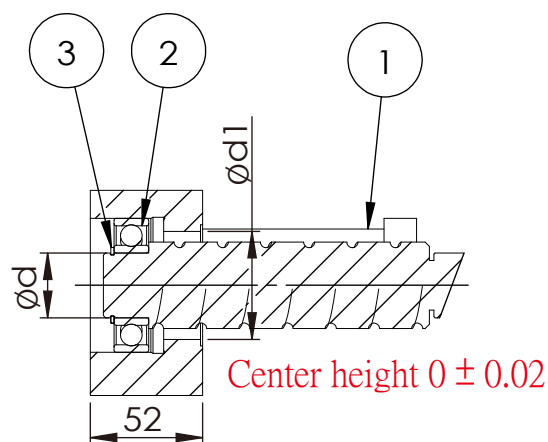
Section H-H
